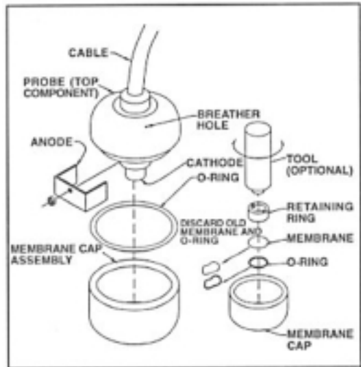
Figure 4.4 OxyGuard DO Probe
