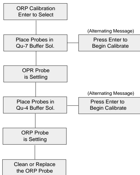
Figure 4.9 ORP Calibration Menu
